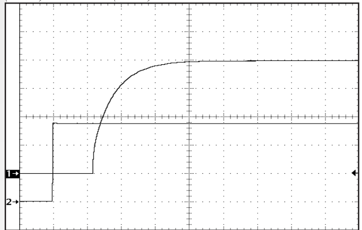
Turn-on transient at full resistive load and zero output capacitance initiated by Vin. ENA1 and ENA2 both previously high. Ch 1: Vout (3V/div). Ch 2: Vin (10V/div).
