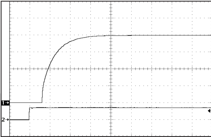
Figure 7: Turn-on transient at full resistive load and zero output capacitance initiated by ENA1. Input voltage pre-applied. Ch 1: Vout (3V/div). Ch 2: ENA (5V/div).
